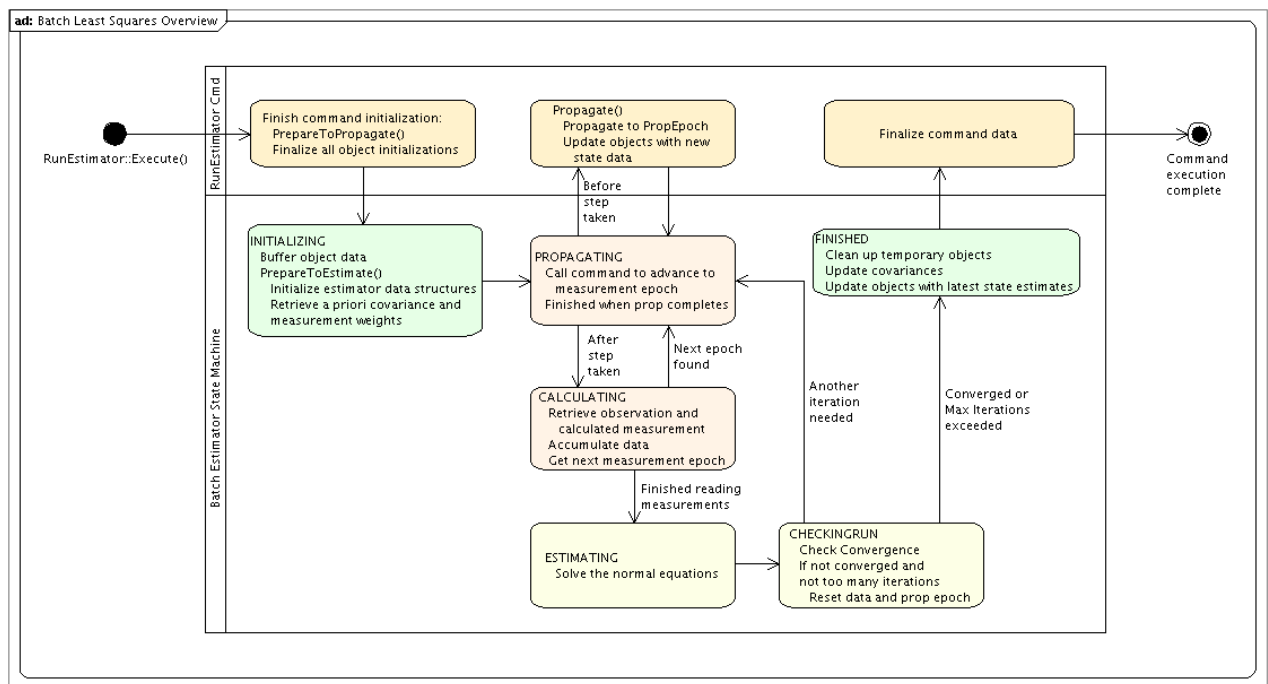
Figure 2.6: Performing Batch Estimation
