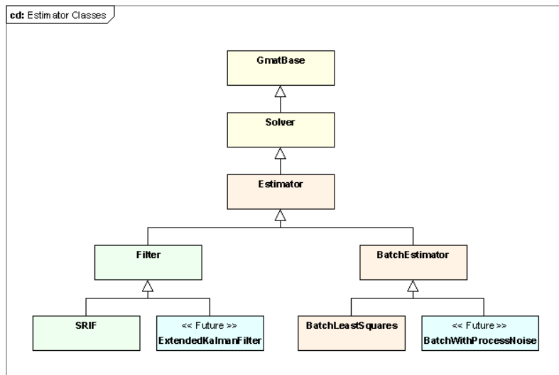
Figure 2.1: Classes in GMAT's Estimator Hierarchy
