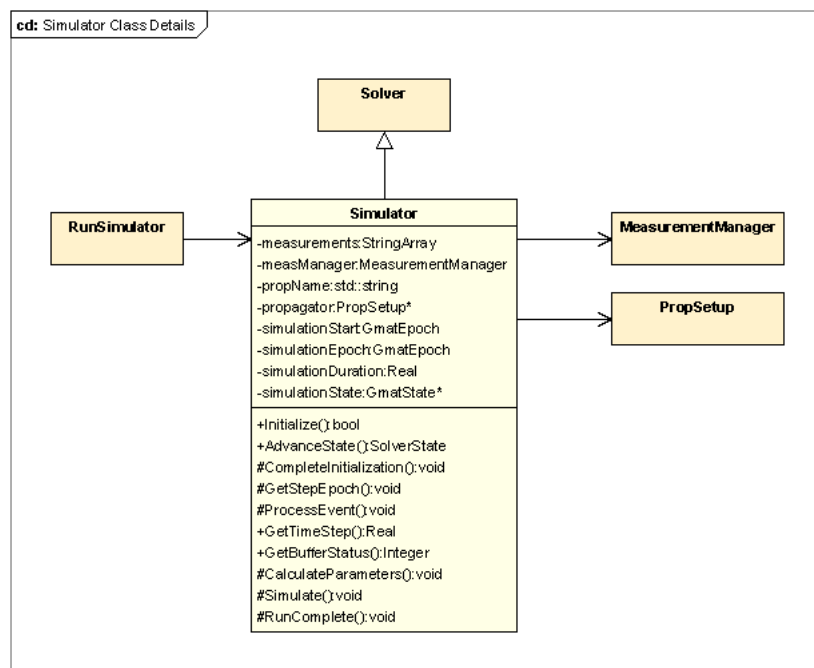
Figure 2.8: The Simulator Class
