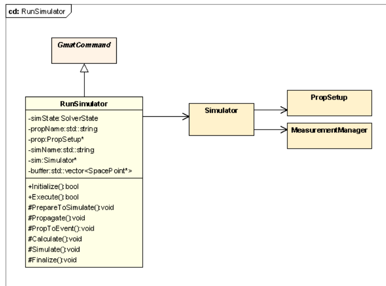
Figure 3.5: The RunSimulator Class
