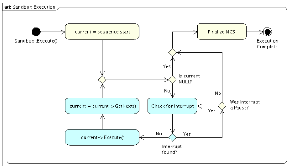
Figure 1.6: The Sandbox::Execute() Method
