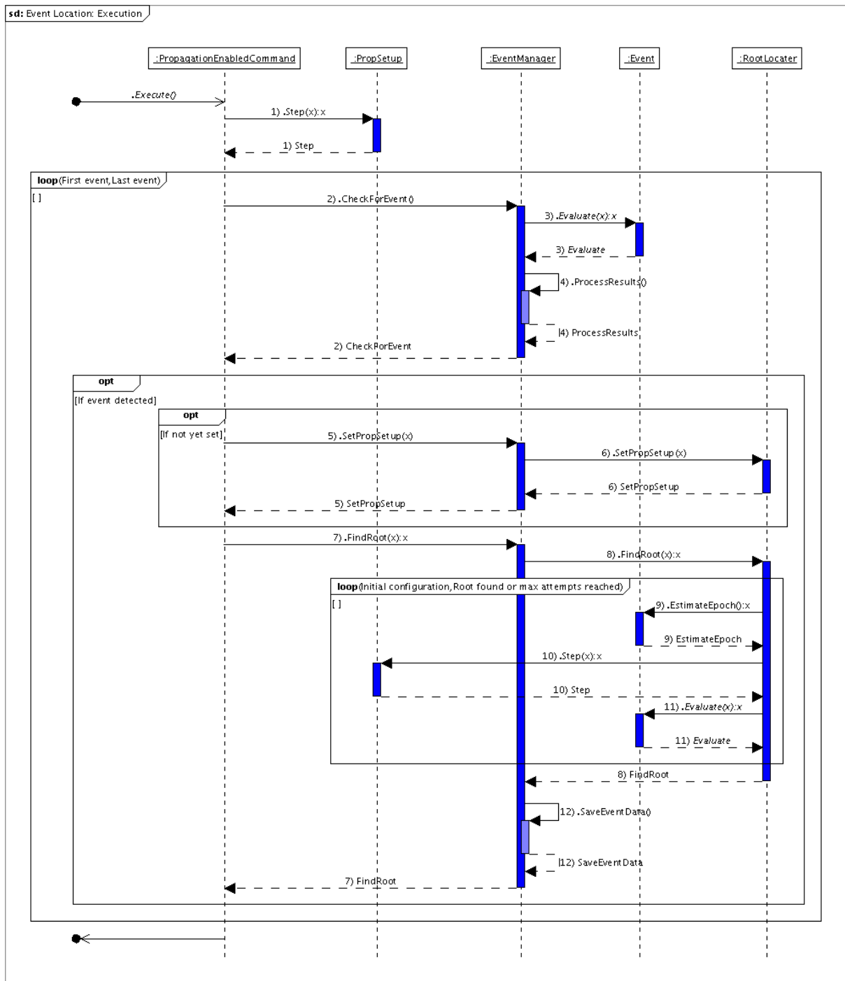
Figure 4.1: The Event Location Process
