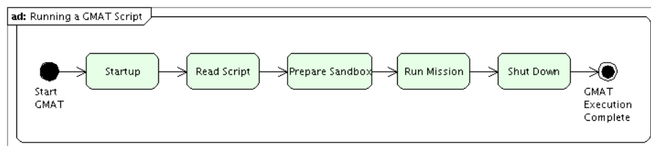
Figure 1.2: GMAT Run Overview – Running a Script
