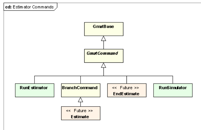
Figure 3.1: Commands Used in Estimation
