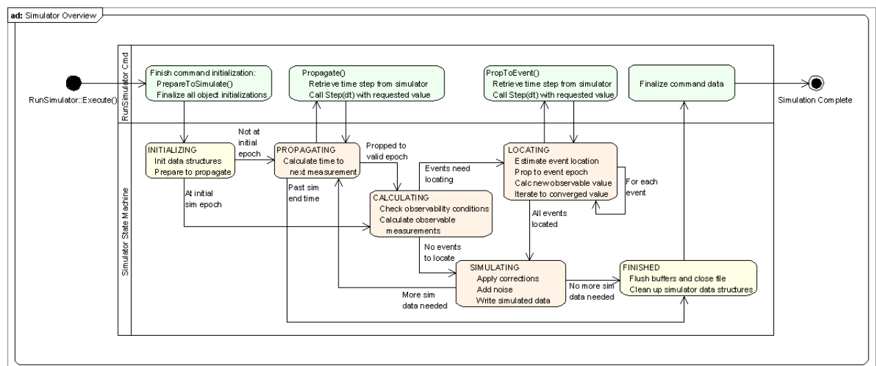
Figure 3.4: The Simulation State Machine
