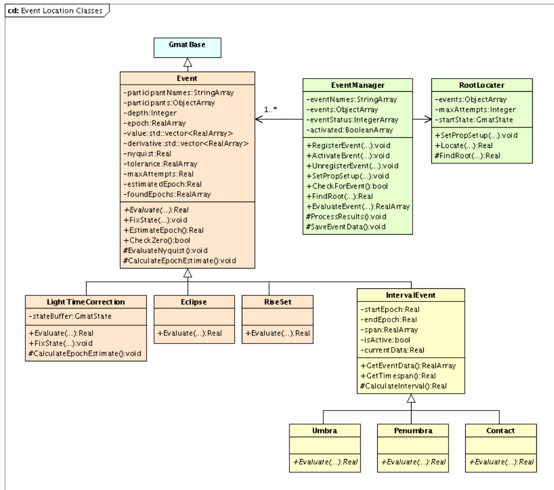
Figure 4.2: Event Location Classes
