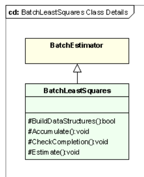
Figure 2.7: The BatchLeastSquares Class
