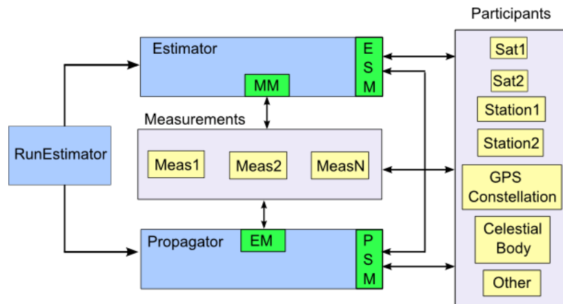
Figure 1.1: OD Components and Interactions
