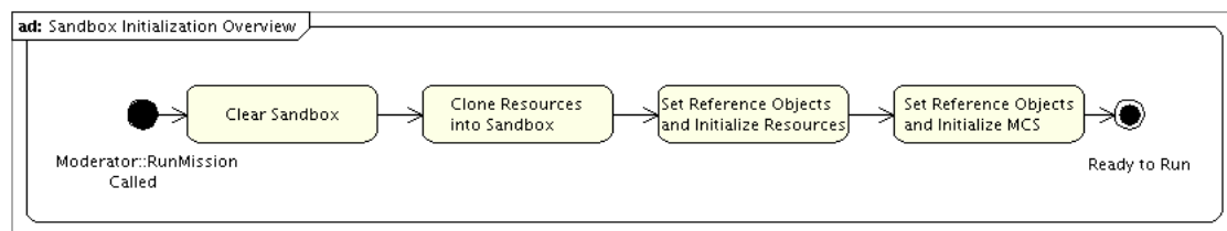
Figure 1.4: Steps if the Sandbox Initialization Process
