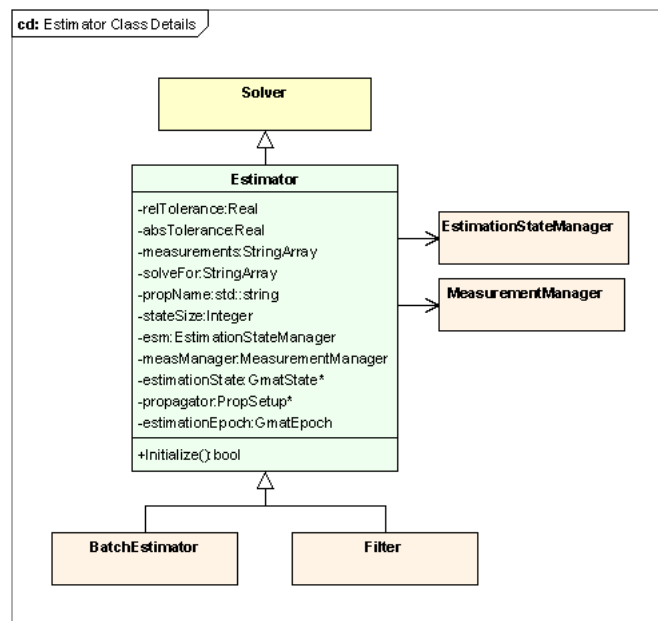
Figure 2.2: The Estimator Class
