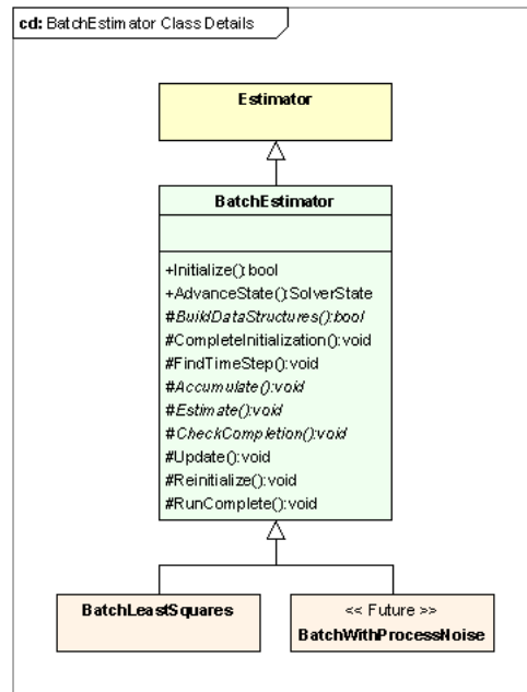
Figure 2.4: The BatchEstimator Class
